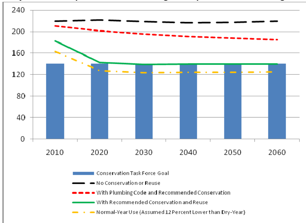
Figure 6.4 Projected Municipal and Manufacturing Per Capita Water Use in Region C
